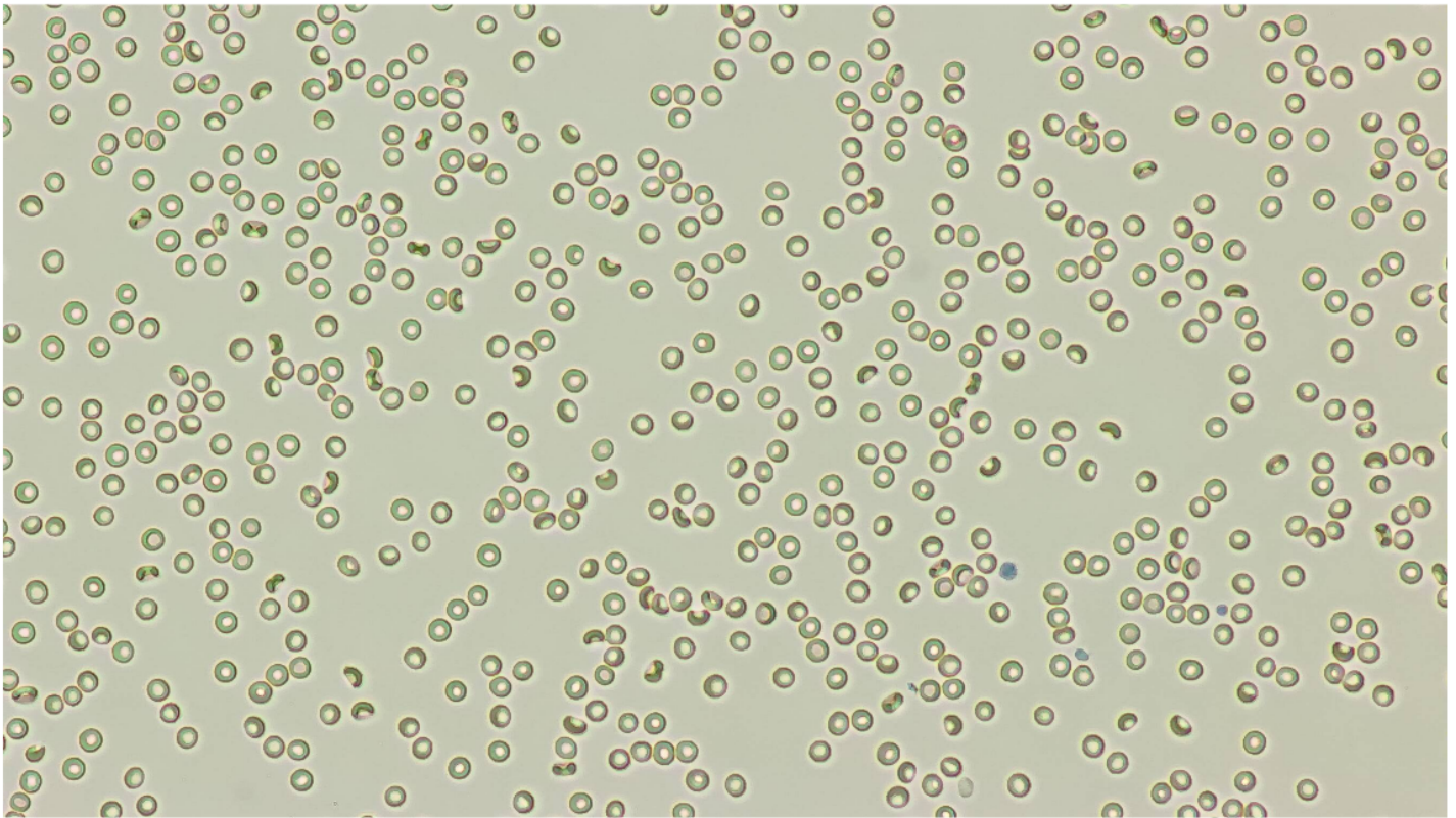
RBC&PLT images
